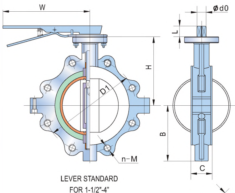
LUG TYPE Series 450L
