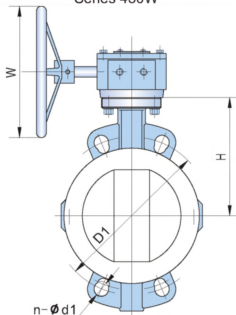
GEAR STANDARD FOR 5" & LARGER
