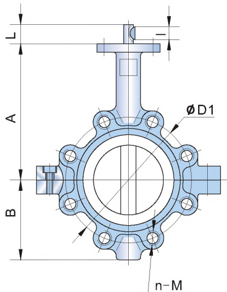
LUG TYPE Series 400L
